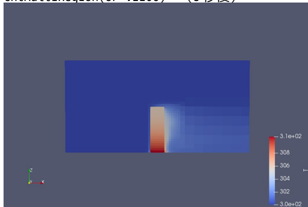
chtMultiRegion(OF-v2206) (3秒後)
