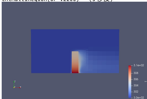
chtMultiRegion(OF-v2206) (3秒後)
